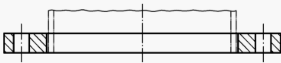
a) Type 01 Plate flange for welding
