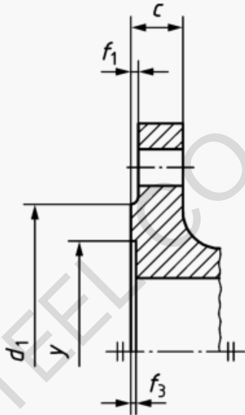
f) Type F: Recess
