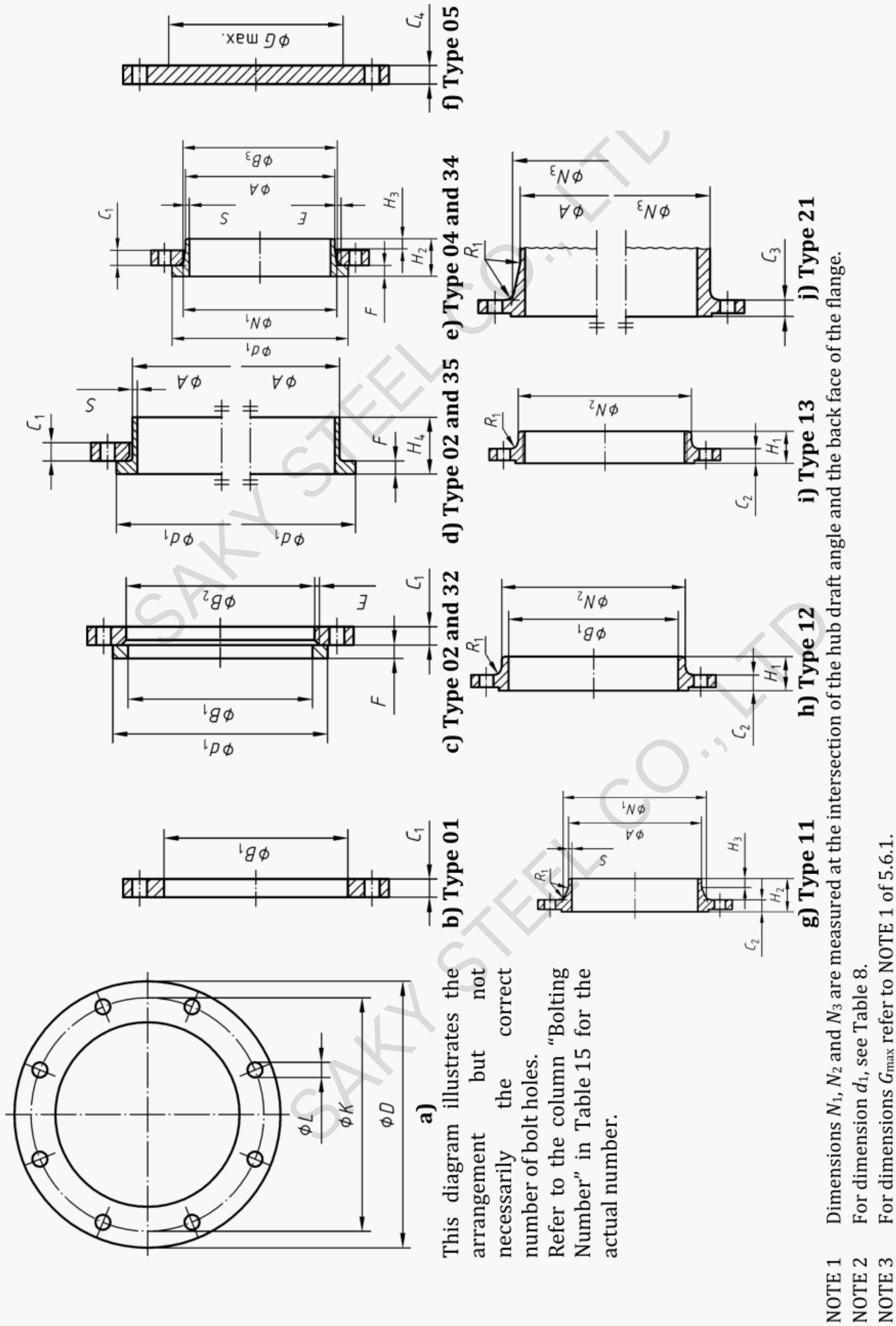
Figure 10 — Dimensions of PN 40 flanges
