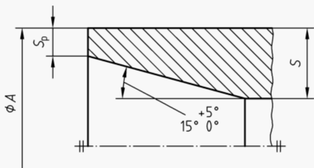
Figure A.4 — Chamfer A for type 35
