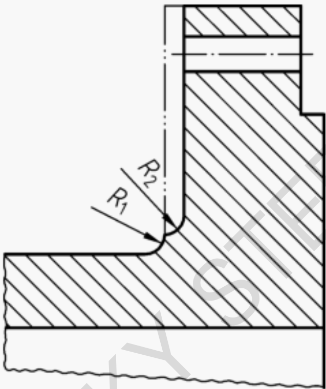
Figure 17 — Minimum hub radius after back facing
