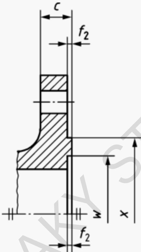
c) Type C: Tongue
