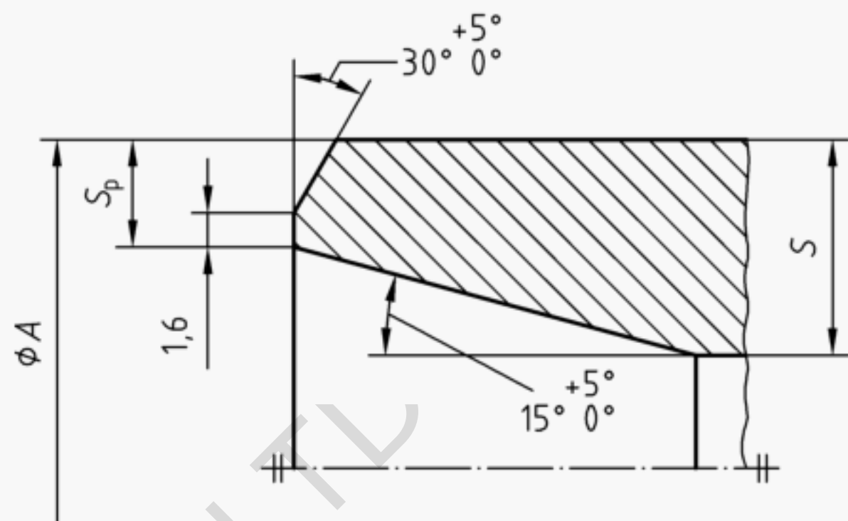
Figure A.5 — Chamfer B for type 35
